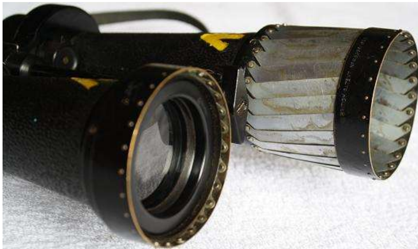
Pict 63, 64; Barr & Stroud CF41 7x50 from James Stewart collection, kindly sent for this article; Copyrights pictures James Stewart
