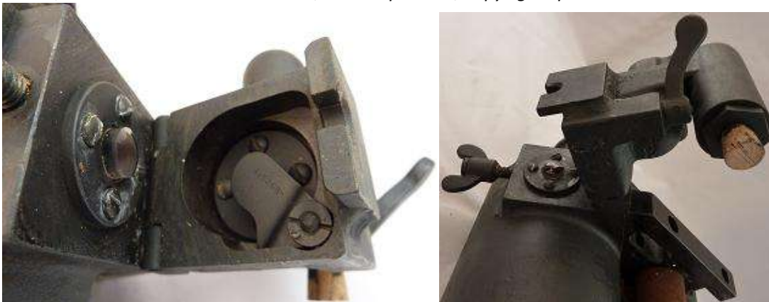
Pict 54; Bausch & Lomb MK 91 Mod 1; the lamp house opened; copyrights pictures Anna Vacani The lamp is to illuminate the reticules (greticule – eng US) in the right ocular are crosshairs.
