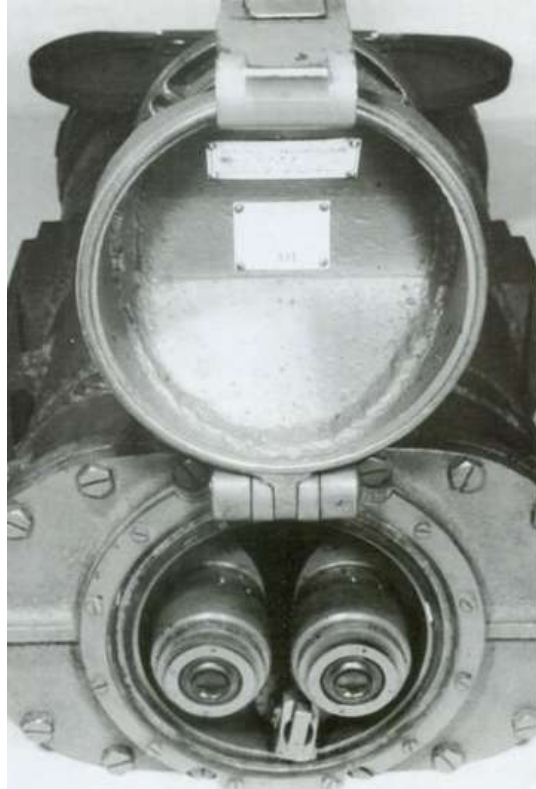
A CLOSER VIEW OF TO REAR WATERTIGHT HATCH WICH IS CONTROLLED BY A LOCKING WHEEL. THE EYEPIECES CAN BE ADJUSTED FOR EYE SEPARATION. ON THE INSIDE SURFACE OF THIS HATCH IS THE IDENTIFICATION PLATE. IT SHOWS A PRODUCTION DATE OF OCTCBER 1944 WITH THE SERIAL NUMBER 311. ALSO PRESENT IS THE NIKKO LOGO USED BY NIPPON KOGAKU; BOTH BEFORE, DURING AND AFTER THE WAR. R. LINE
