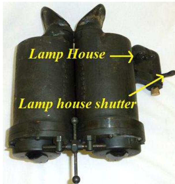
Pict 53; Bausch & Lomb MK 91 Mod 1; the lamp house; copyrights pictures Anna Vacani
